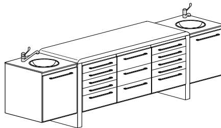
Art. TC7 W 268 / D 55 / H 97
