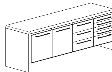
Art. TC12 W 218 / D 55 / H 97 W 50 / D 55 / H 200 sink unit
