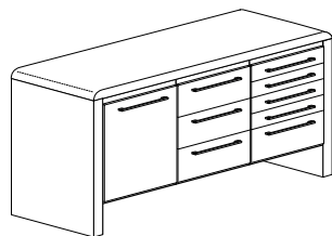
Art. TC10 W 168 / D 55 / H 97 W 50 / D 55 / H 200 sink unit
